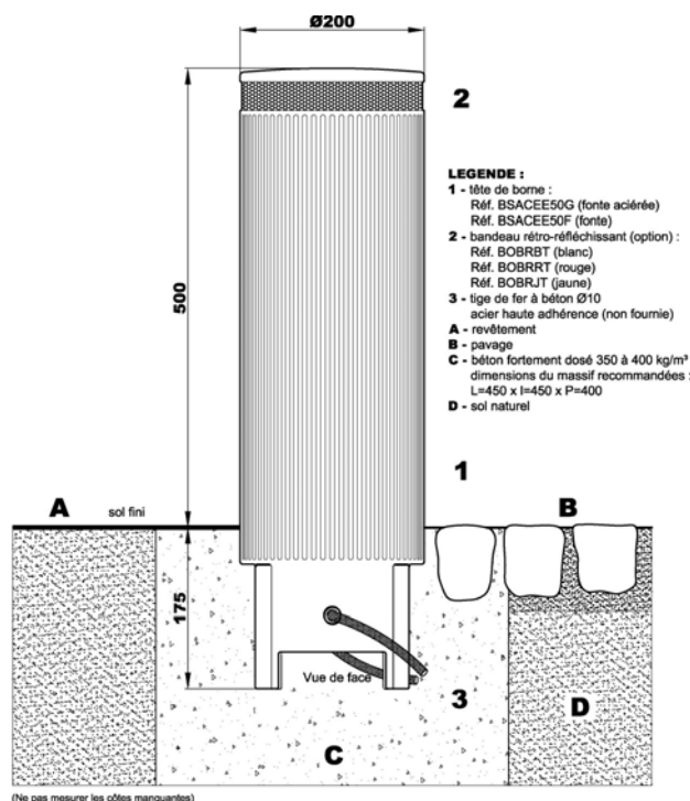
Acropole bollard head
