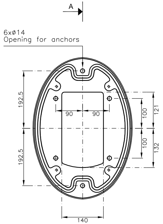
Socle 3AEM5S02 Top view
